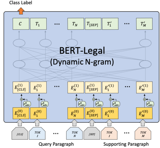
Figure 4: The detailed illustration of the fine-tuning BERT-Legal (+FGM) model.
